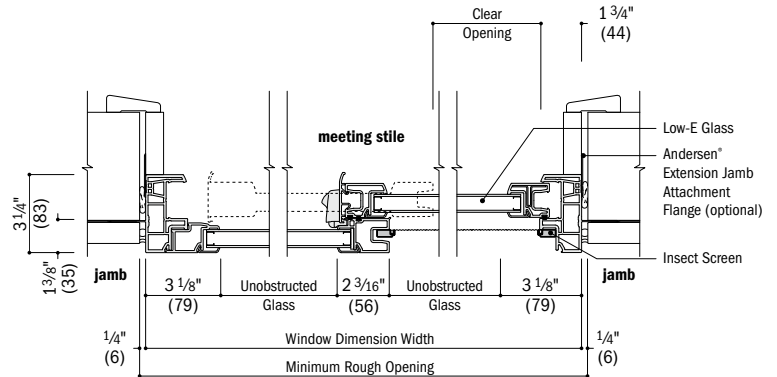
Horizontal Section
