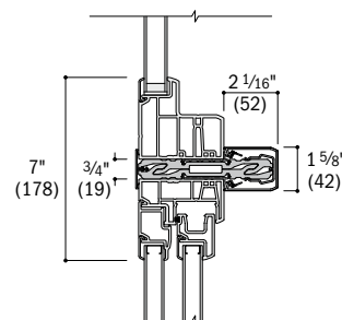
Picture/Single Transom/Specialty over Gliding
