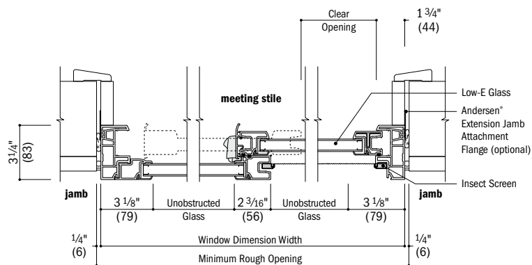
Horizontal Section existing framed opening
