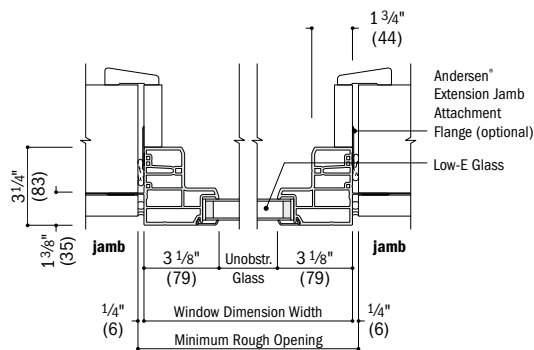
Horizontal Section
