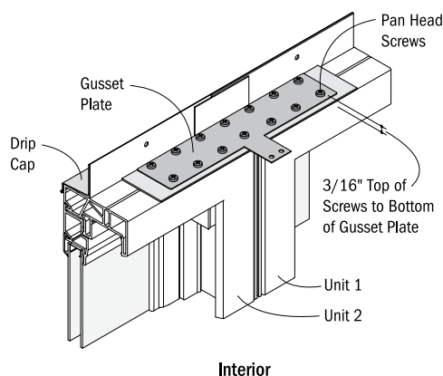
Example of two units joined together with the use of gusset plates and pan head screws that will require additional rough opening space. Rough opening for joined units must be a minimum of 3/4" (19) plus the overall joined window dimensions.
