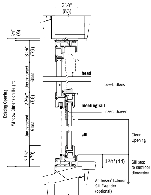
Vertical Section
