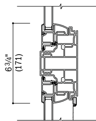
Vertical Section Picture over Awning
