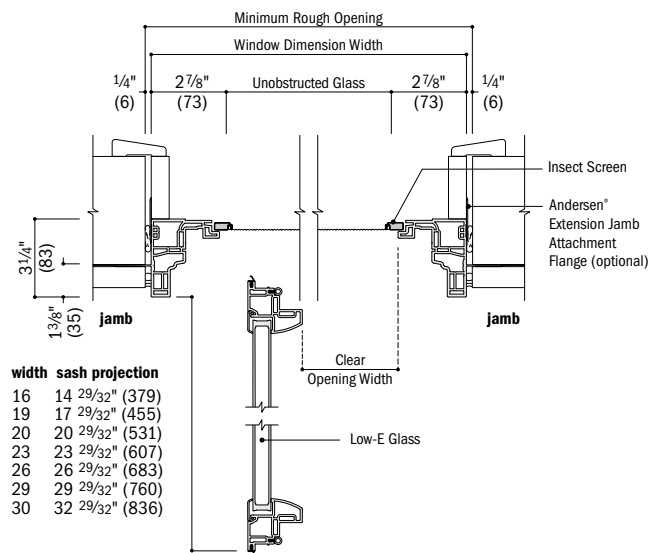
Horizontal Section
