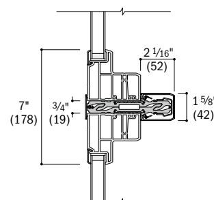
Picture/Single Transom/Specialty over Picture/Single Transom
