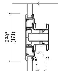
Vertical Section
